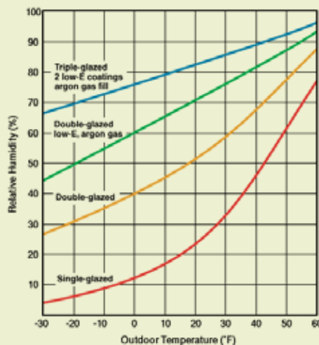
This chart illustrates condensation curves for various window configurations.
